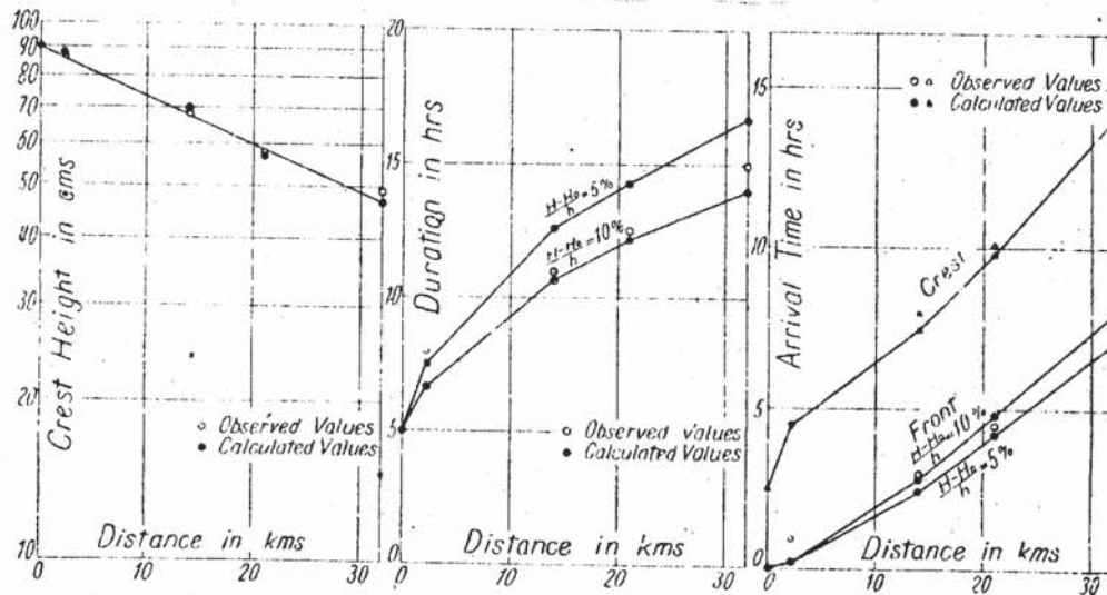
Fig. 3. Comparison of observational results with theoretical computation (solitary unit flood in the Yedo River).
