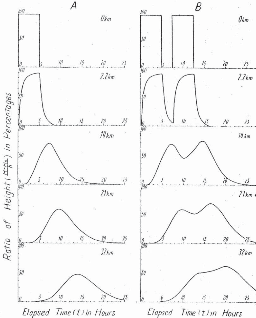
Fig. 1-A. Propagation of a solitary unit flood. Fig. 1-B. Propagation of two successive unit floods.
