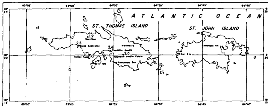
FIGURE 4-59.—10-yr. 30-min. rainfall for Virgin Islands (in.).
