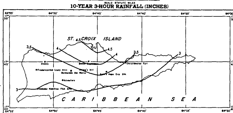
FIGURE 4-80.—10-yr. 3-hr. rainfall for Virgin Islands (in.).
