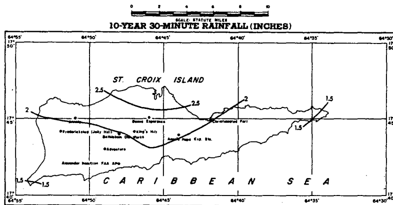
FIGURE 4-59.—10-yr. 30-min. rainfall for Virgin Islands (in.).
