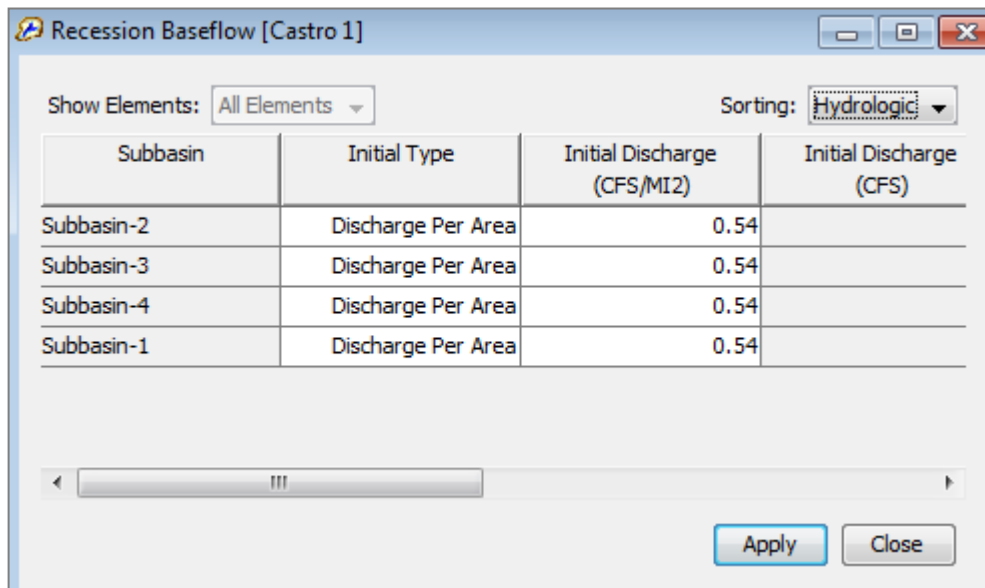
Figure 35. Recession baseflow global editor.
