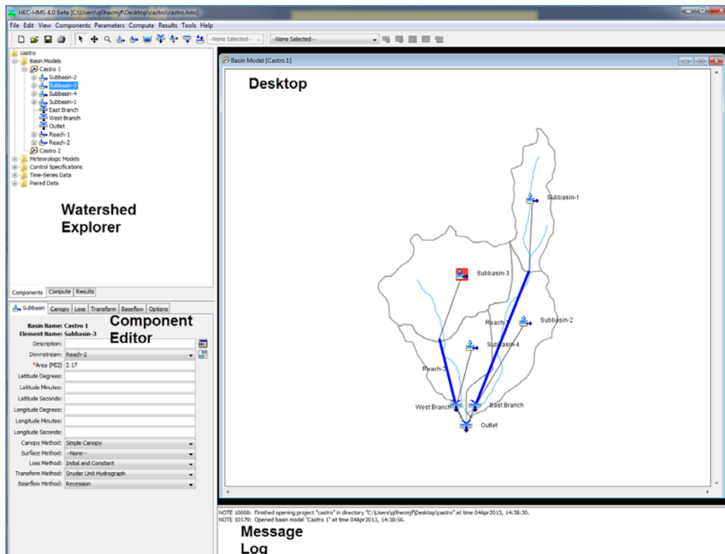
Figure 1. HEC-HMS user interface.
