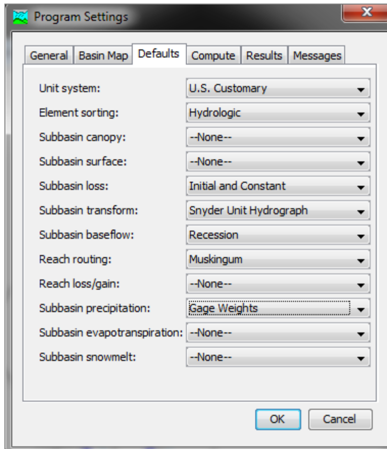
Figure 27. Setting the program settings.
