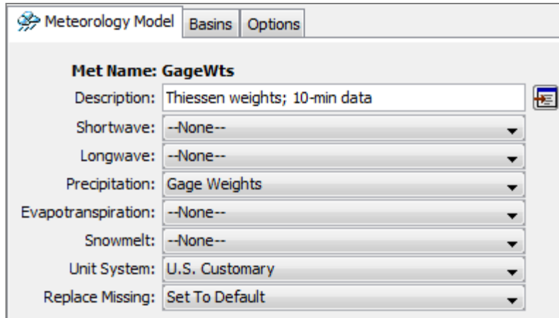
Figure 16. Component editor for a meteorologic model.
