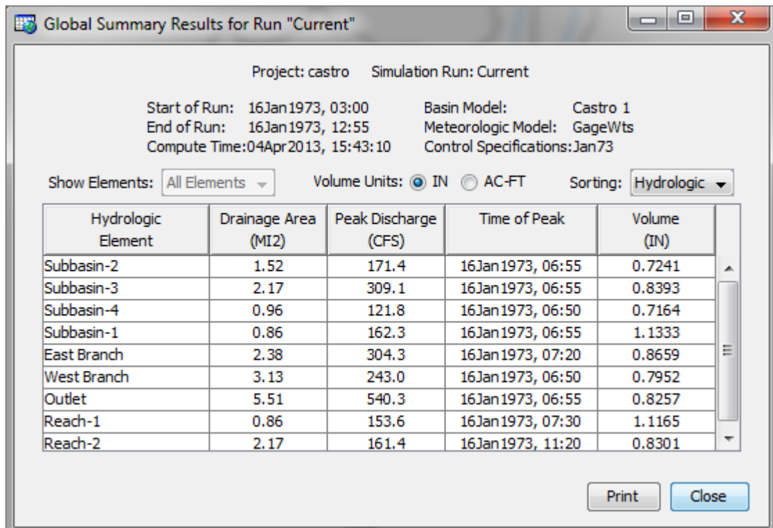
Figure 49. Viewing the global summary table.
